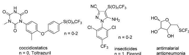
Figure 1. Examples of SCF 3 -containing pharmacologically active compounds.
